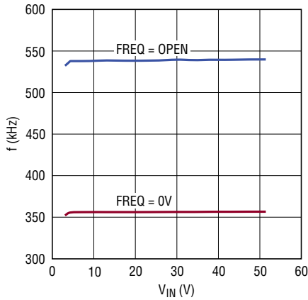
Frequency Over Input Voltage
