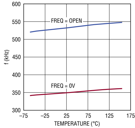
Frequency Over Temperature
