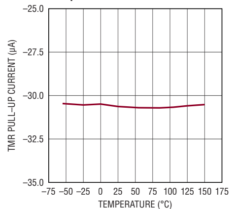
TMR Pull-Up Current Over Temperature
