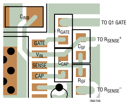
Figure 8. LTC7860 Recommended Gate Driver PC Board Placement, Layout and Routing
